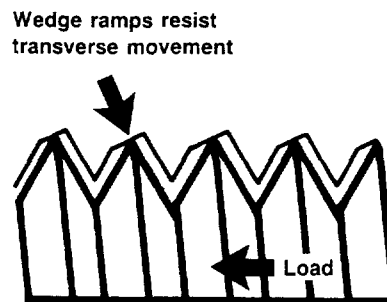
Figure 1.—Spirallock thread.
